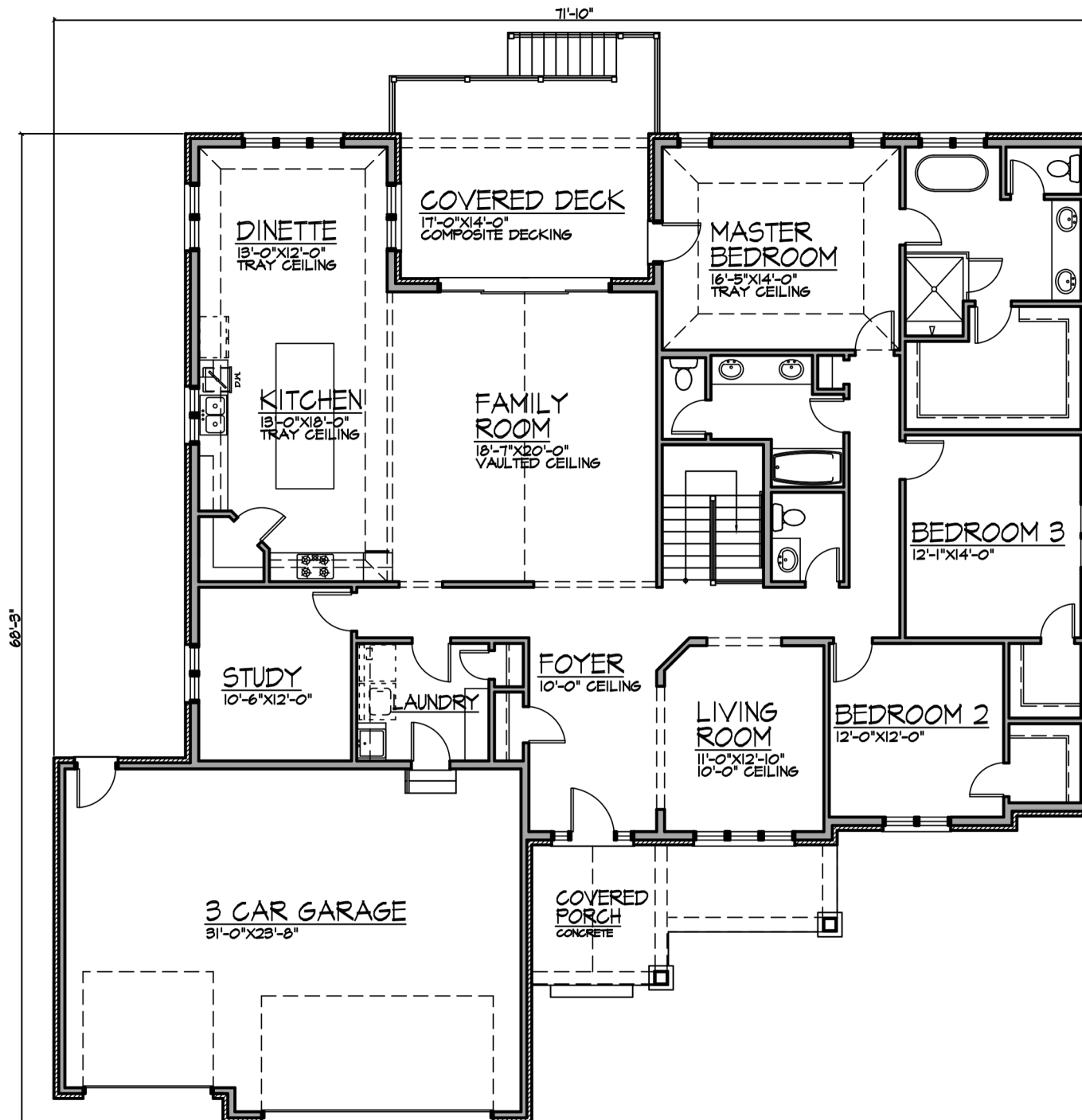
First Floor Plan 2,761 Total Square Feet
