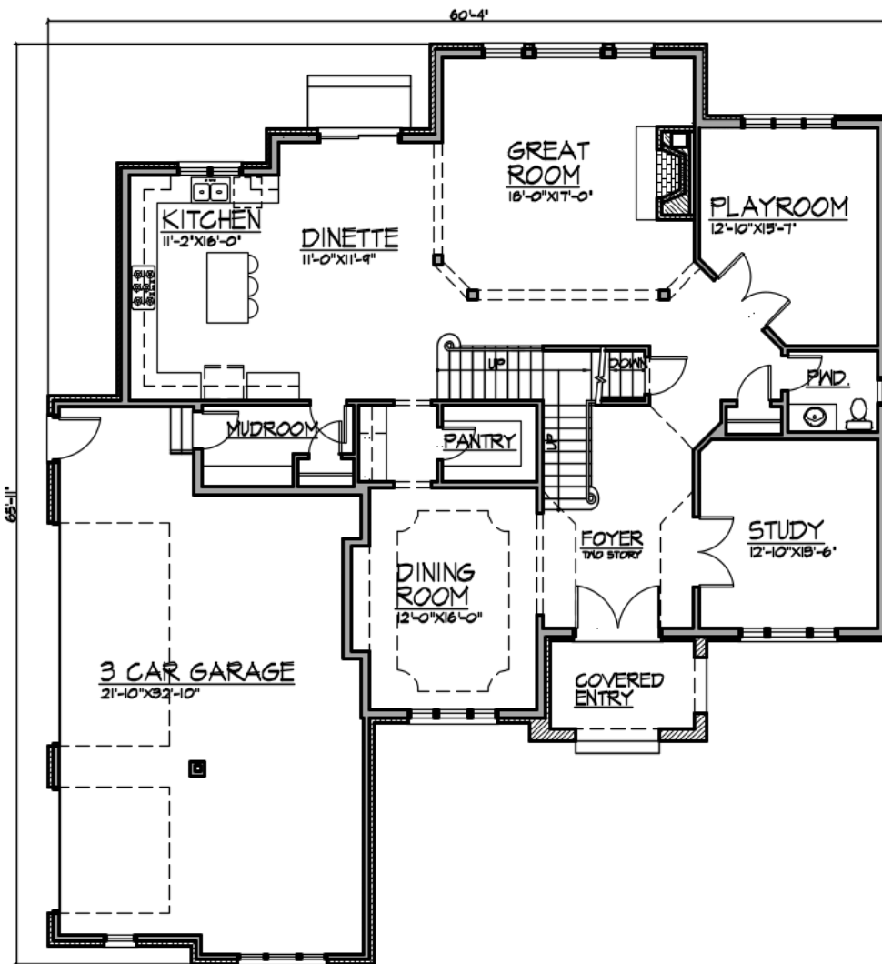
First Floor Plan 3,783 Total Square Feet
