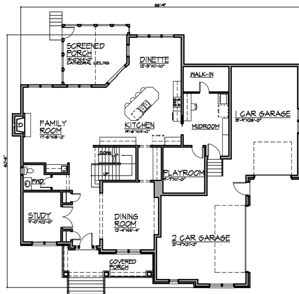
First Floor Plan 3,915 Total Square Feet
