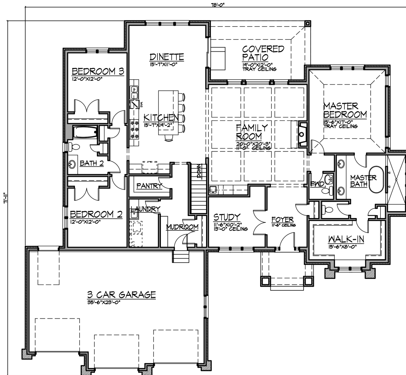
First Floor Plan 2,754 Total Square Feet
