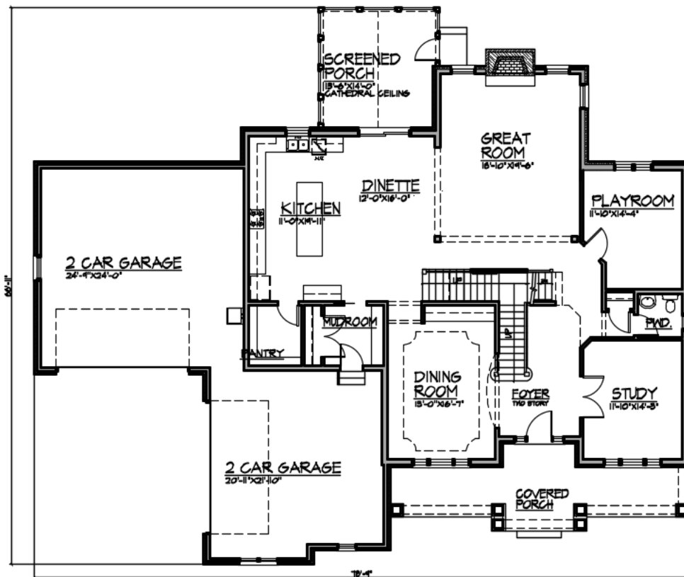
First Floor Plan 4,307 Total Square Feet
