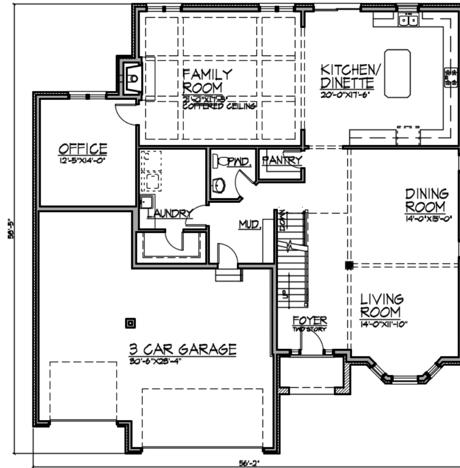
First Floor Plan 3,762 Total Square Feet
